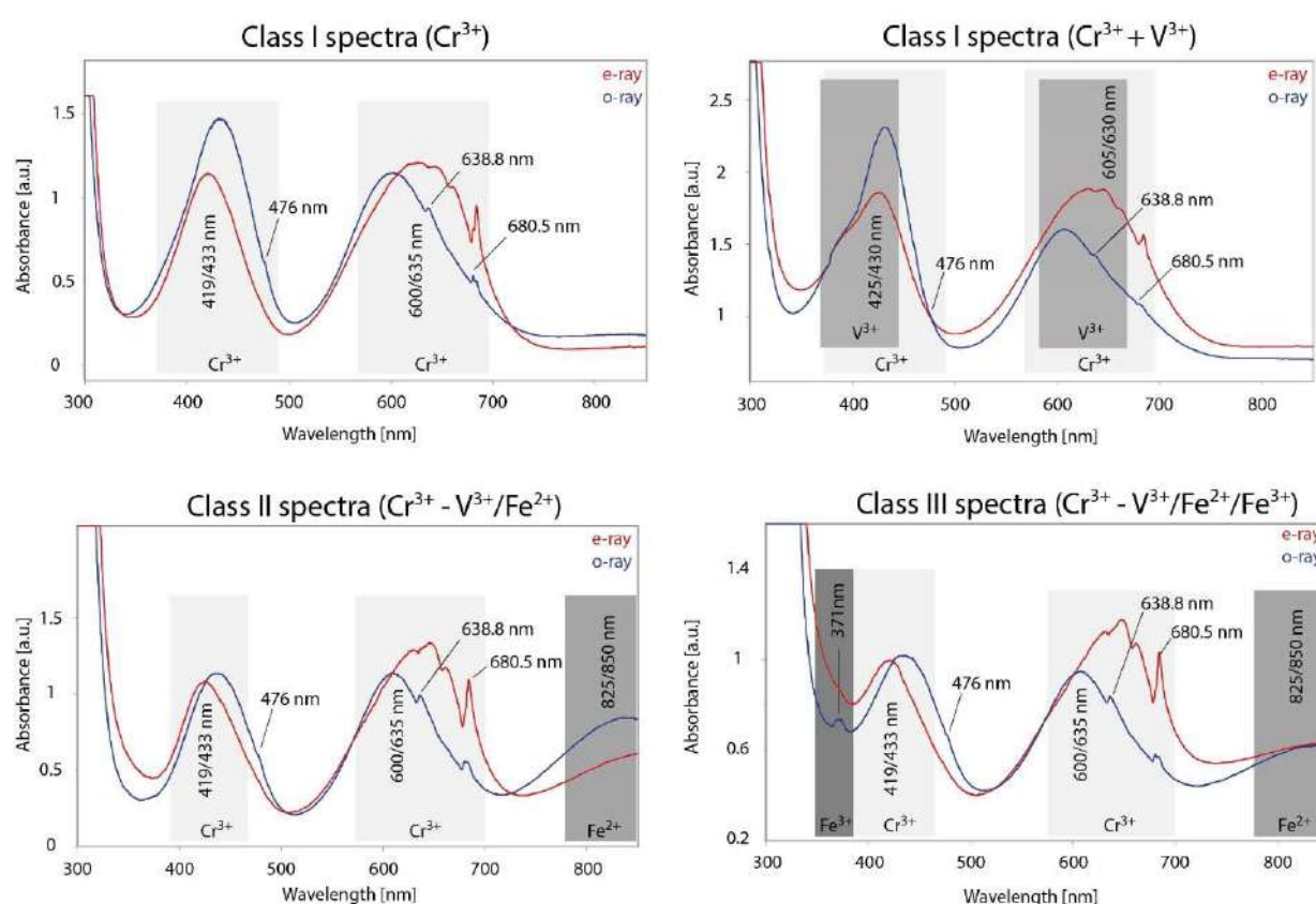
Figure 2: UV-Vis-NIR absorbance graphs for spectral classification in Smith (2009) (modified after original data). Class I shows \text{Cr}^{3+} absorption only, or with \text{V}^{3+} . Class II shows the absorption of \text{Cr}^{3+} and potentially \text{V}^{3+} , and various \text{Fe}^{2+} absorption depending the source. Class III shows the combination of the absorption of \text{Cr}^{3+} , potentially \text{V}^{3+} and both oxidation state of iron. Class IV (not represented in the article) is the rare combination of \text{V}^{3+} only and both oxidation state of iron.
