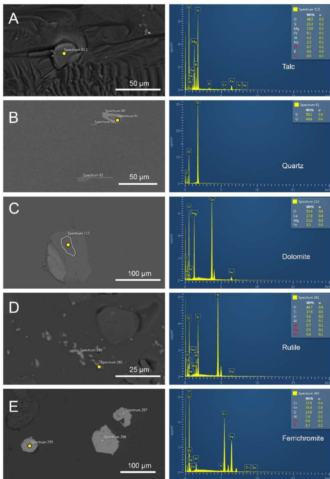
Figure 46: BSE pictures and compositions of inclusions in emerald samples. A Grain of talc as inclusion, with nickel traces (FN12970, BSE, crushed). B A quartz intergrowth with two muscovite platelets (FN12974, BSE, polished). C Dolomite crystal with minor siderite content (FN12974, BSE, polished). D Rutile grains on a crystal face (FN12973, BSE, polished). E (V-Zn)-ferrichromite flakes (FN12976, BSE, polished).
