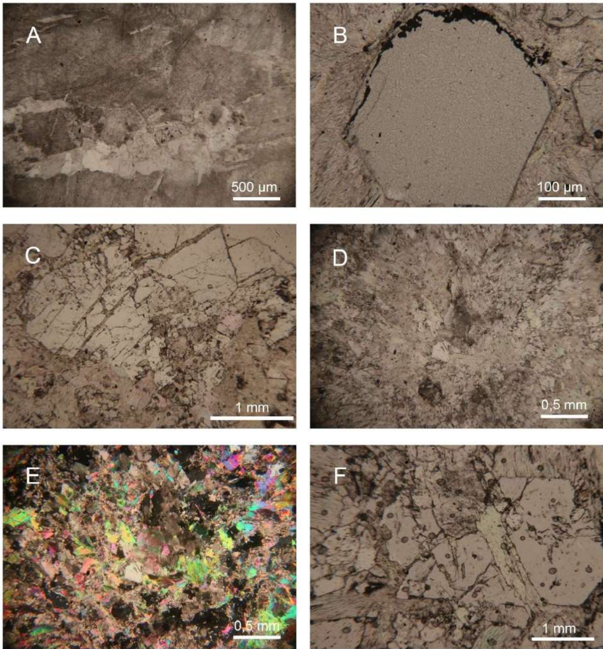
Figure 41: A emerald-quartz-muscovite veinlets cross-cutting the large-grained magnesite domain (LC-khalid-8, PPL). B A basal section of emerald in the fine magnesite-talc matrix. The black pinpoints inclusions on the rims of the emerald are oxides (LC-khalid-8, PPL). C Fractured emeralds along cleavage planes pervaded by fine magnesite, within a magnesite-talc-muscovite-dolomite matrix (LC-khalid-9, PPL). D General view (LC-khalid-9, PPL). E Same general view (LC-khalid-9, XPL). F An emerald crystal replaced by muscovite-magnesite (LC-khalid-9, PPL).
