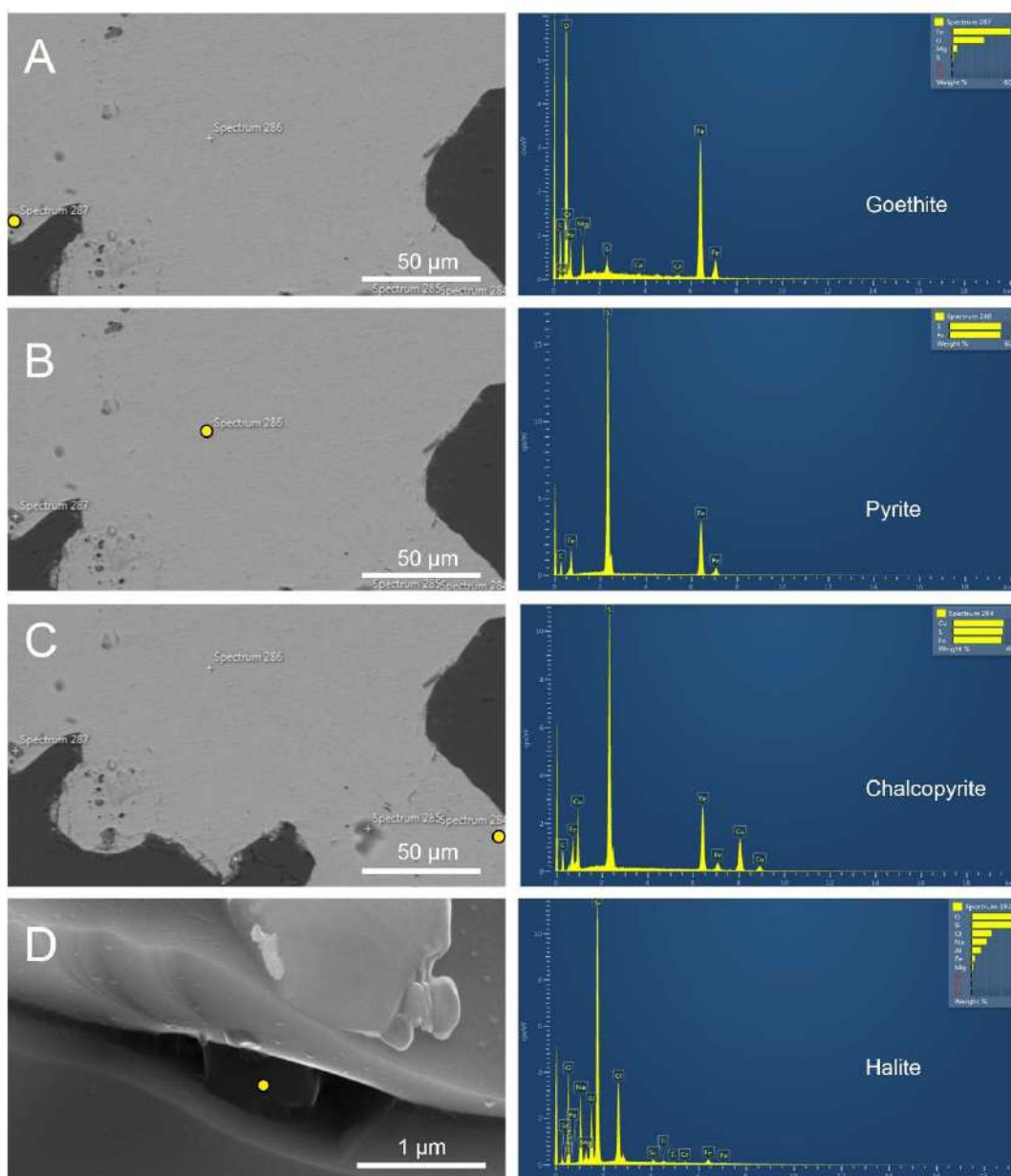
Figure 47: BSE pictures and compositions of inclusions in emerald samples. A A grain of goethite trapped in the middle of a large pyrite grain (FN12975, BSE, polished). B A large pyrite grain (FN12975, BSE, polished). C Chalcopyrite replacing the pyrite grain (FN12975, BSE, polished). D Cubic halite crystal still trapped in an empty multi-phase fluid inclusion (FN12970, SE, crushed).
