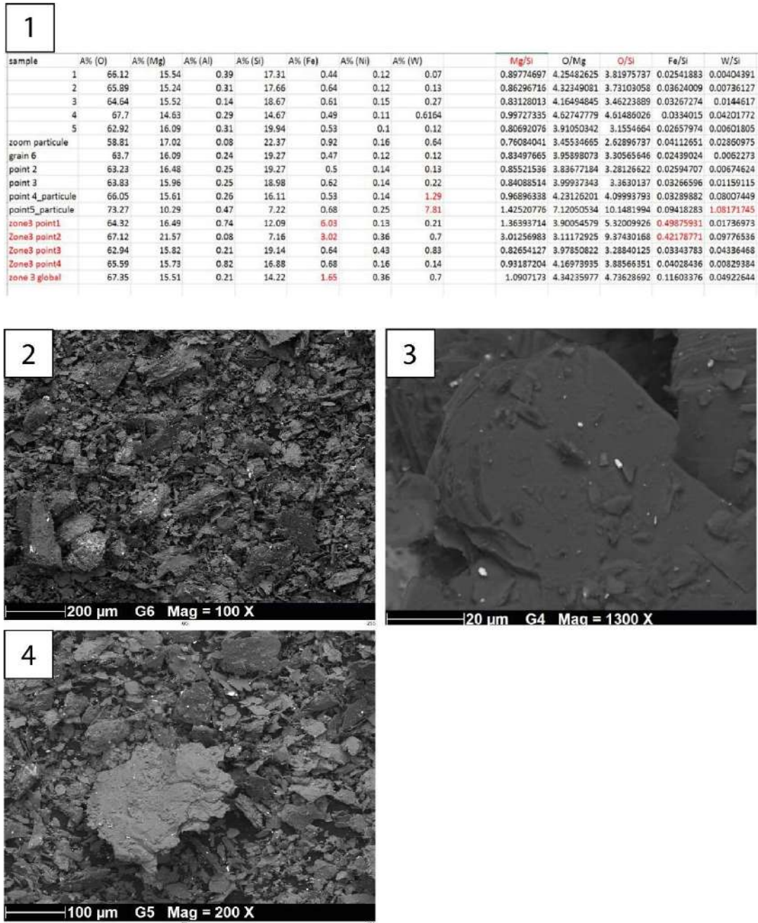
Figure 48: EDX-SEM results for the analyses on the rock samples. 1) Table of the completed qualitative analyses with EDX-SEM on the powders of LC-center-1, LC-center-2, LC-khalid-2 rock samples. The Mg-Si-O composition of the grains displays large range of Mg/Si ratio, it could be a mix of derivated pyroxenes ( \text{MgSiO}_3 ) and talc ( \text{Mg}_4\text{Si}_3\text{O}_{12} ) with variable Mg/Si ratio. 2) Platy shapes of the particles influences the qualitative analyses cited above (sample LC-center-2). 3) Another view of the sample LC-center-2. 4) The smaller and denser grains on the platy minerals is potentially a contamination during the sampling (sample LC-center-2).
