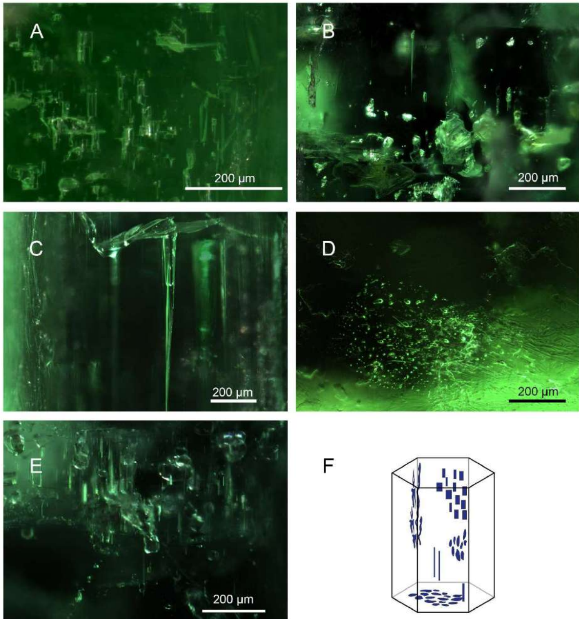
Figure 16 Primary and secondary fluid inclusions. A Blocky two-phase fluid inclusions, aligned along the C-axis (FN12976, ethanol, darkfield). B Negative crystals, growth spikes (up) along with «repeated growth-restrictions» (Gübelin and Koivula, 1997) forming comb-like inclusions (bottom) (FN12968, ethanol, darkfield). C Bigger biphas growth spike inclusion (FN12968, ethanol, darkfield). D Secondary monophas and two-phase inclusions, the result of a healed fissure (FN12490, ethanol, darkfield). E Batch of small xenomorph transparent crystals coupled with growth tubes and curved alignment of secondary inclusions (bottom) (FN12968, ethanol, darkfield). F Sketch illustrating the different primary and secondary inclusions found in Mingora emeralds.
