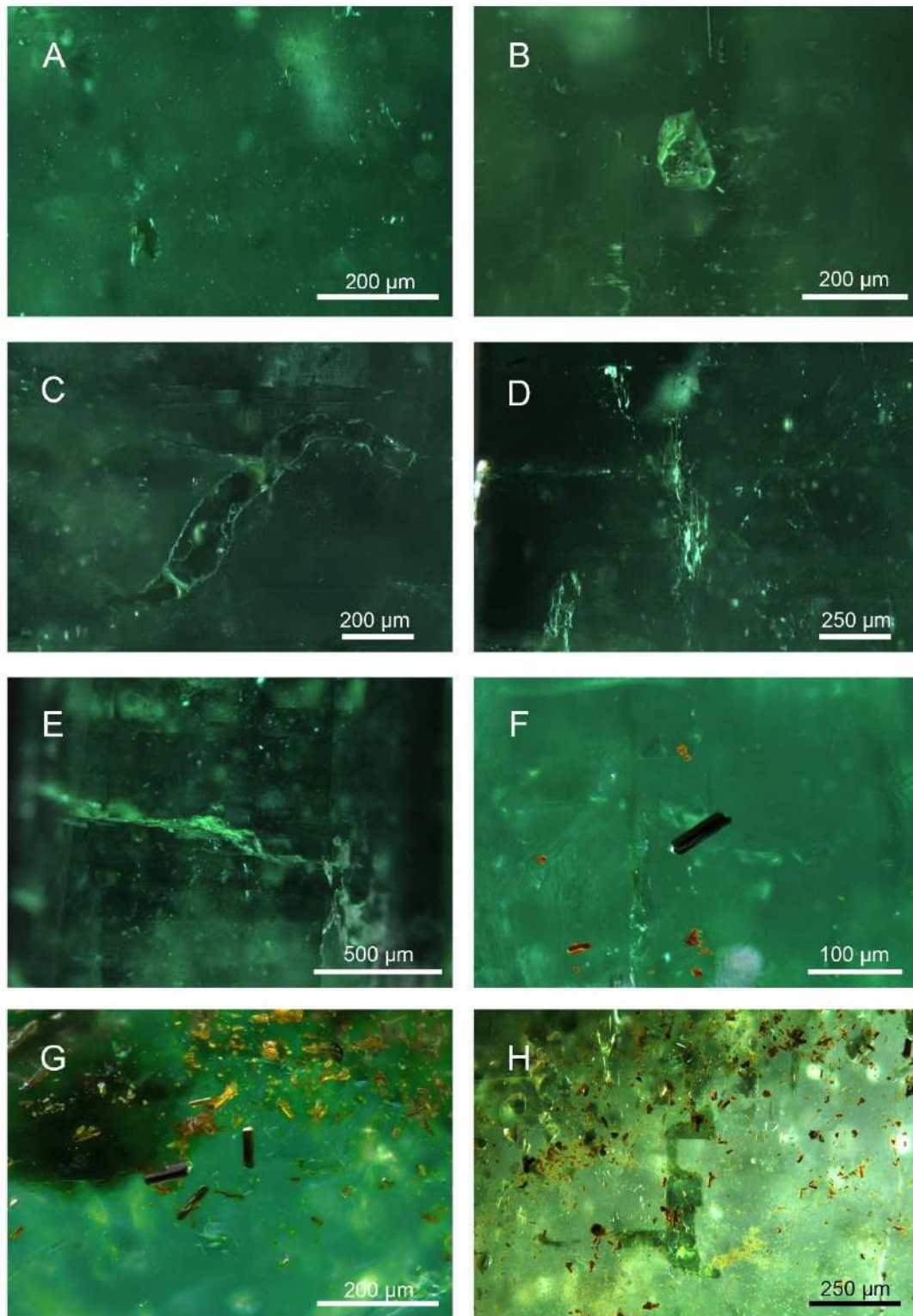
Figure 27: A A cloud of fluid inclusions coupled with few micas sheets (FN12491-3, ethanol, darkfield). B A dolomite crystal with elongated fluid inclusions, biphasic growth spike and growth-restrictions comb (FN12491-5, ethanol, darkfield). C Undulating chlorite sheet, close to the crystal face (FN12491-7, ethanol, darkfield). D Jagged primary fluid inclusions plane and visible cleavage plane on the crystal surface (FN12491-8, ethanol, darkfield). E Late fracture following the cleavage planes through the sample (FN12491-11, ethanol, darkfield). F Black acicular crystal of rutile with smaller grains around (FN12969-2, ethanol, brightfield). G Black acicular crystals of rutile with smaller cluster of grains around (FN12969-5, ethanol, brightfield). H Orange rutile grains of different size and saturation, and geometrical thin sheet of chlorite following cleavage planes and primary fluid inclusion plane (FN12969-6, ethanol, brightfield).
