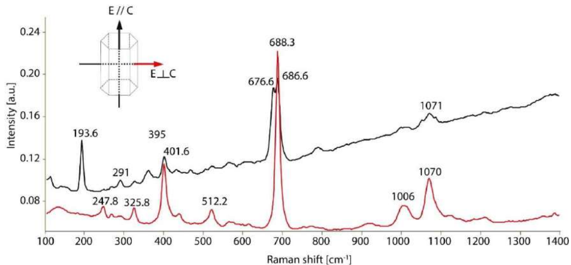
Figure 22: Absorbance Raman spectrum for the FN12491 sample
