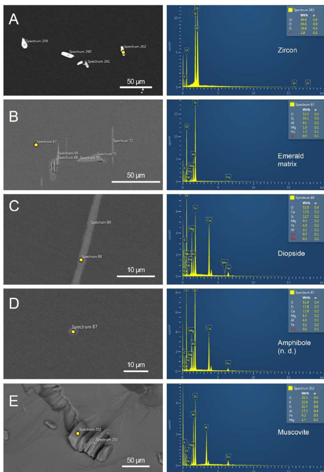
Figure 44: BSE pictures and compositions of inclusions in emerald samples. A Zircon grains on a crystal face with minor micro-inclusions of xenotime/apatite, due to minor phosphorus content (FN12969, BSE, polished). B An analysis's point in emerald matrix (FN12974, BSE, polished). C A side-view of flat sheet of diopside (FN12974, BSE, polished). D A perpendicular cut rod of undefined amphibole (omphacite-jadeite, clinopyroxene, tschermakite) (FN12974, BSE, polished). E Muscovite forming as columnar crystals (FN12970, BSE, crushed).
