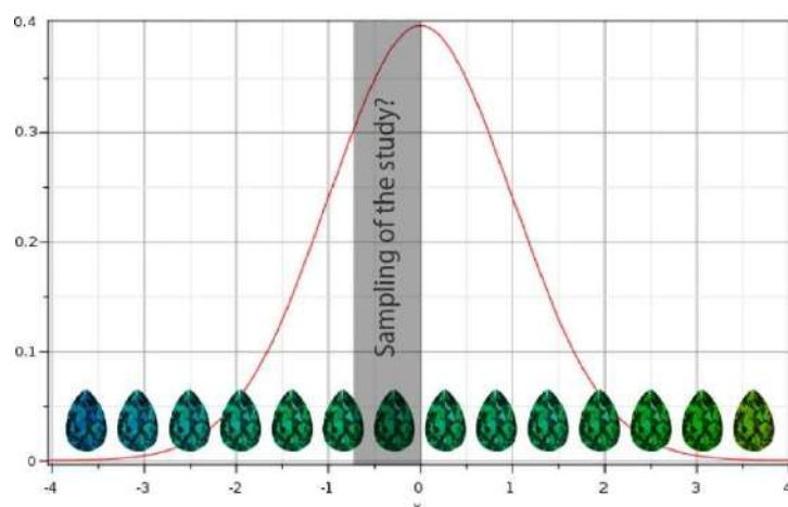
Figure 3: Theoretical gaussian distribution of the color of gems extracted from a single deposit. The selection bias will generalize the color for the whole deposit only based on the few collected samples (modified after Franck Notari's talk during DUG sessions).
