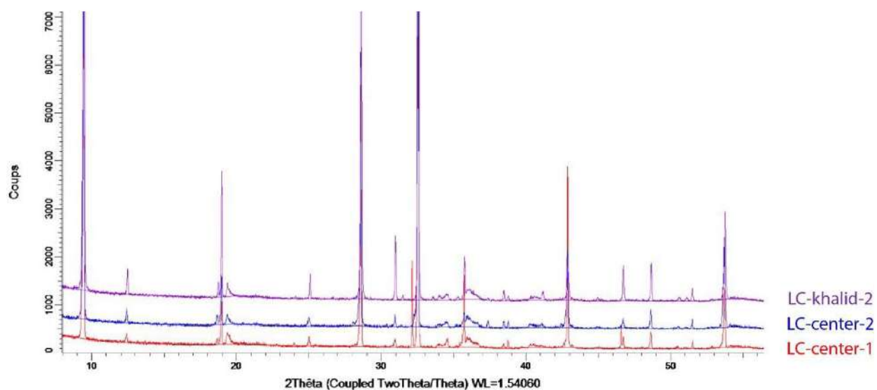
Figure 43: ED-XRD pattern for 3 powders of fault breccias selected out the rock sampling batch.
