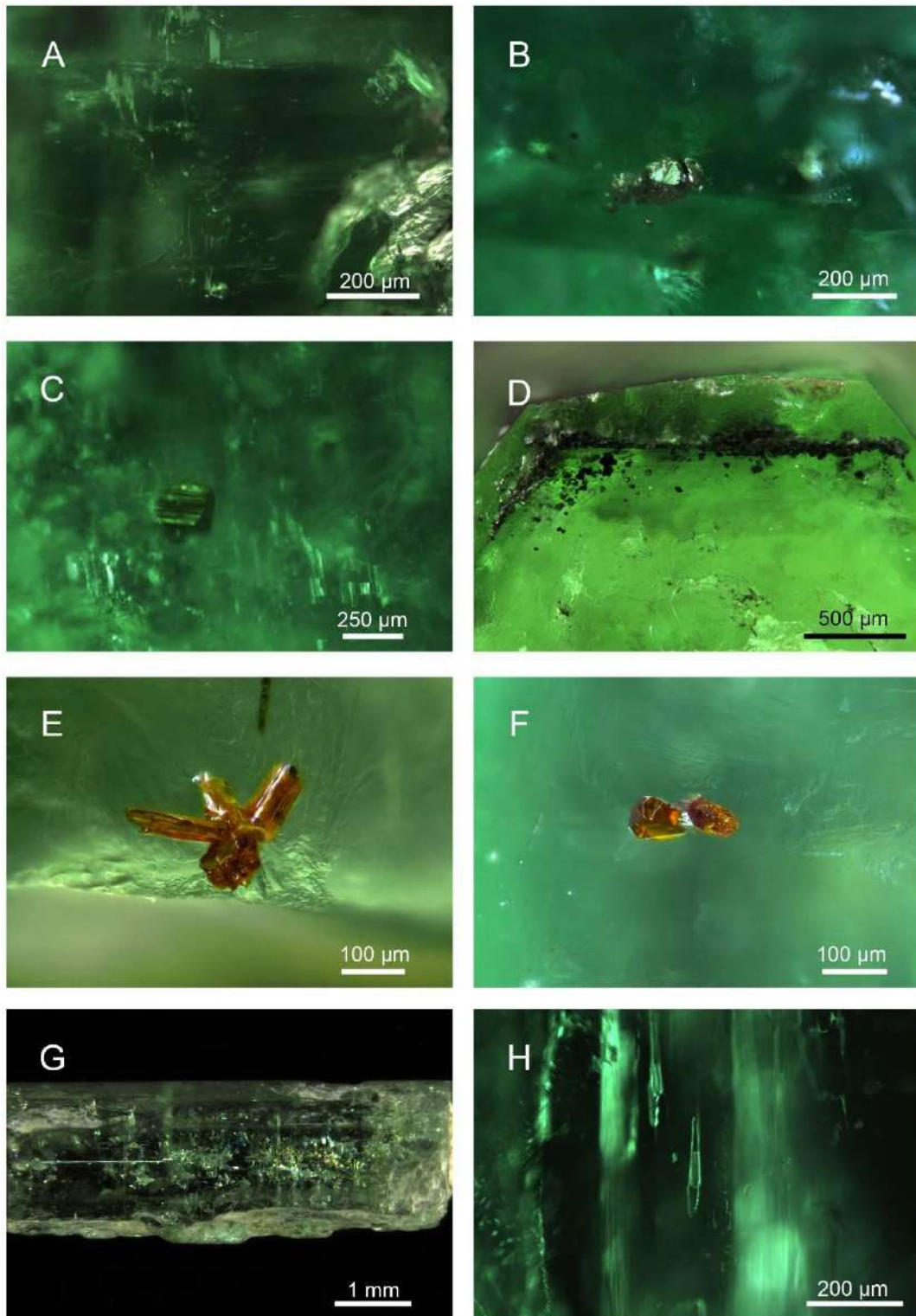
Figure 29: A A jagged primary fluid inclusions plane (FN12975-4, ethanol, darkfield). B A pseudo-octahedral pyrite grain in aggregate with smaller ones (FN12975-6, ethanol, darkfield). C Striated pseudo-euhedral pyrite grain surrounded by a cloud of minute fluid inclusions and blocky two-phase inclusion //C (FN12976-3, ethanol, darkfield). D Layers of «sharp chromites» flakes (Kazmi and Snee, 1990, Gübelin and Koivula, 2008) restricted on a single crystallization plane \perp C view (FN12976-5, ethanol, darkfield). E Twinning of rutile (FN12979-2, ethanol, darkfield). F Twinning of rutile (FN12979-3, ethanol, darkfield). G Unidentified accordion-like micas in the center of a crystal; the diffraction colors are created by the different micas crystal planes (FN12981-2, ethanol, darkfield). H Two elongated biphase fluid inclusions //C (FN12984-4, ethanol, darkfield).
