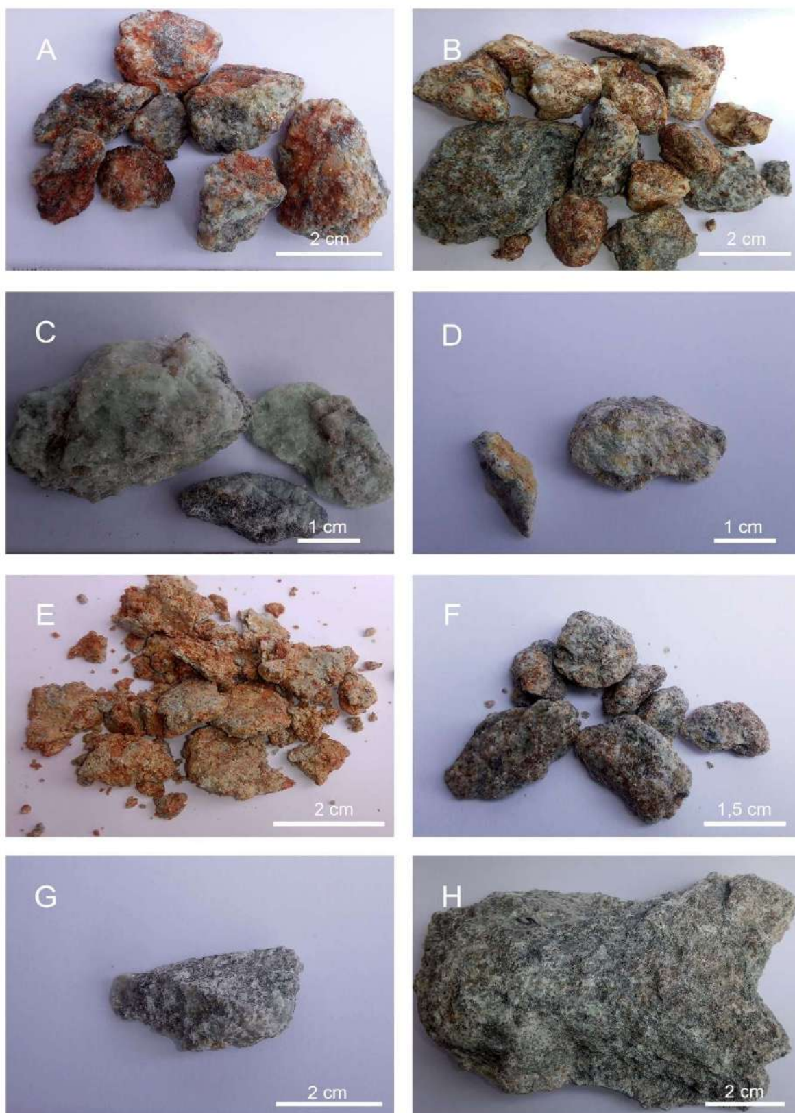
Figure 31: A Alteration near a fault (Wall, LC-center-1). B Alteration near a fault (Wall, LC-center-2). C Talc near mineralization (Wall, LC-center-3). D Talc-magnesite schist without mineralization (Wall, LC-khalid-1). E Altered talc schist next to a fault zone, close to the working face (Wall, LC-khalid-2). F Altered talc schist next to a fault zone, close to the working face (Wall, LC-khalid-3). G Talc schist at the working face (Wall, LC-khalid-4). H Mineralized section (Wall, LC-khalid-5).
