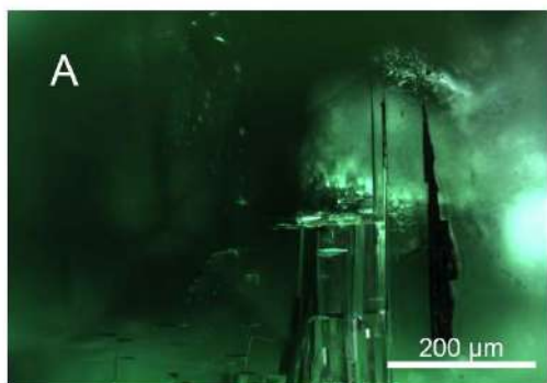
Figure 30: A Flat fluid inclusions and growth restrictions (FN12984-6, ethanol, darkfield).
