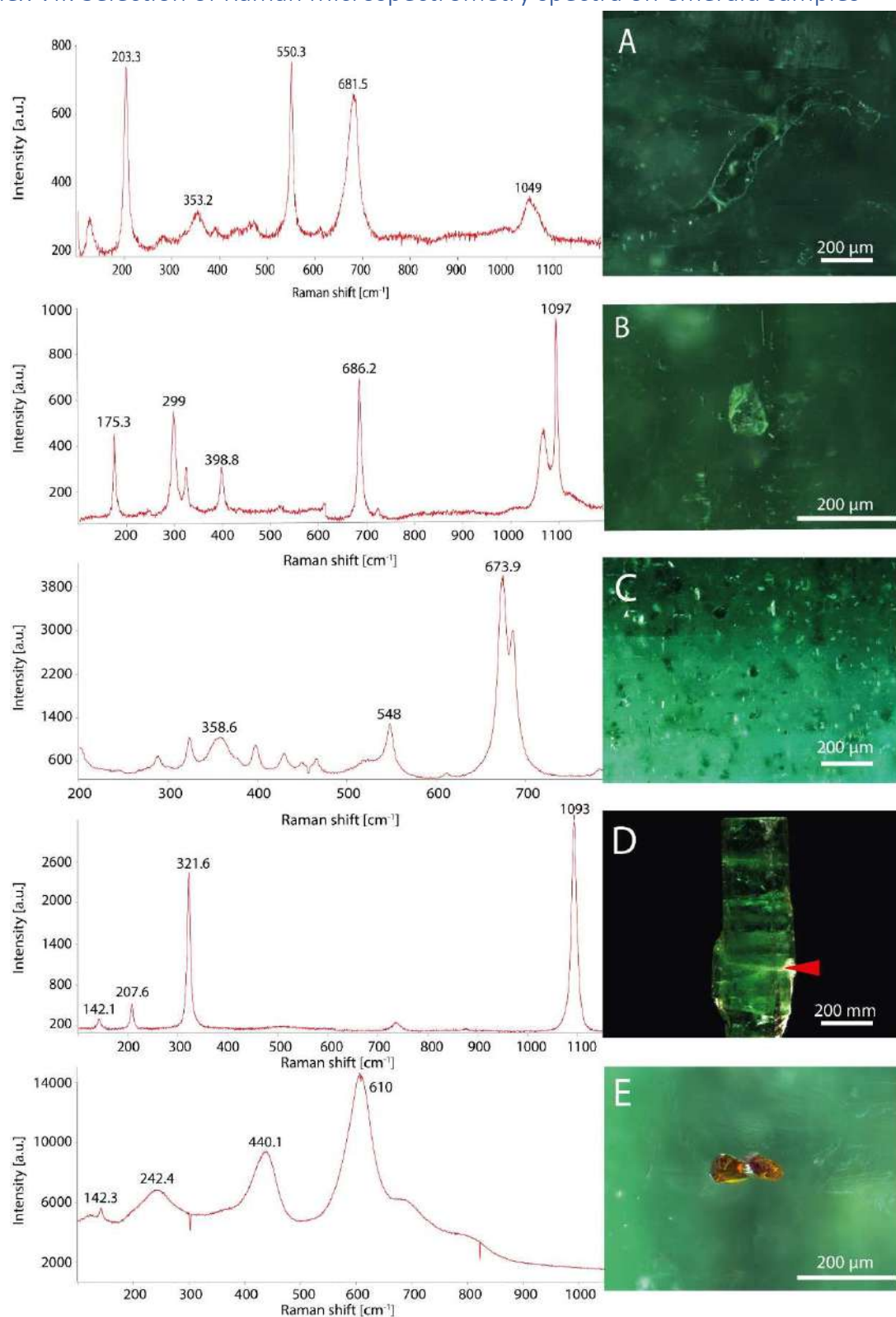
Figure 38: All the spectra are unprocessed or unmodified by any kind of smoothing techniques. A Difficult spectral signature of this thin clinochlore sheet (FN12491, polished). B Spectral signature of a dolomite grain deep inside the crystal (FN12491, polished). C Phlogopite cloud also detected by Raman signature (FN12970, polished). D Magnesite filling spectrum on that rough crystal face (FN12972, rough). E Rutile twins near the surface producing a clear spectrum (FN12979, rough).
