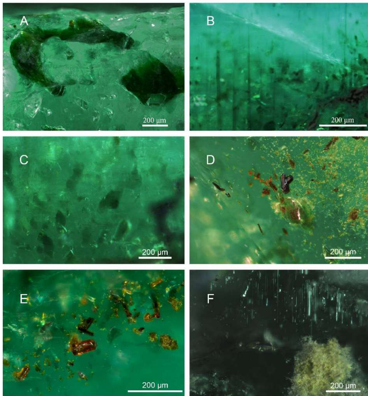
Figure 14: Solid inclusions (chlorite group and rutile). A Chlorite on an unpolished prismatic face (FN12980, ethanol, darkfield). B Elongated chlorite lamellas oriented //C (FN12970, ethanol, darkfield). C Same cluster of «rounded and fuzzy Cr-chlorite» (Gübelin and Koivula, 2008), deeper in the sample (FN12970, ethanol, darkfield). D Two mineralogical types of rutile; a mossy yellowish-white aggregate and acicular, orange to black crystals, with common twins (FN12969, ethanol, brightfield). E Acicular twins of rutile close to the crystalline face, note the color shift between the grains due to REE content (GGTL Lab, personal communication) (FN12969, ethanol, brightfield). F Mossy yellowish-white rutile aggregate with rectilinear growth tubes (FN12973, ethanol, darkfield). Some of the darker mossy aggregates found could be iron-tinted magnesite (Gübelin and Koivula, 1997).
