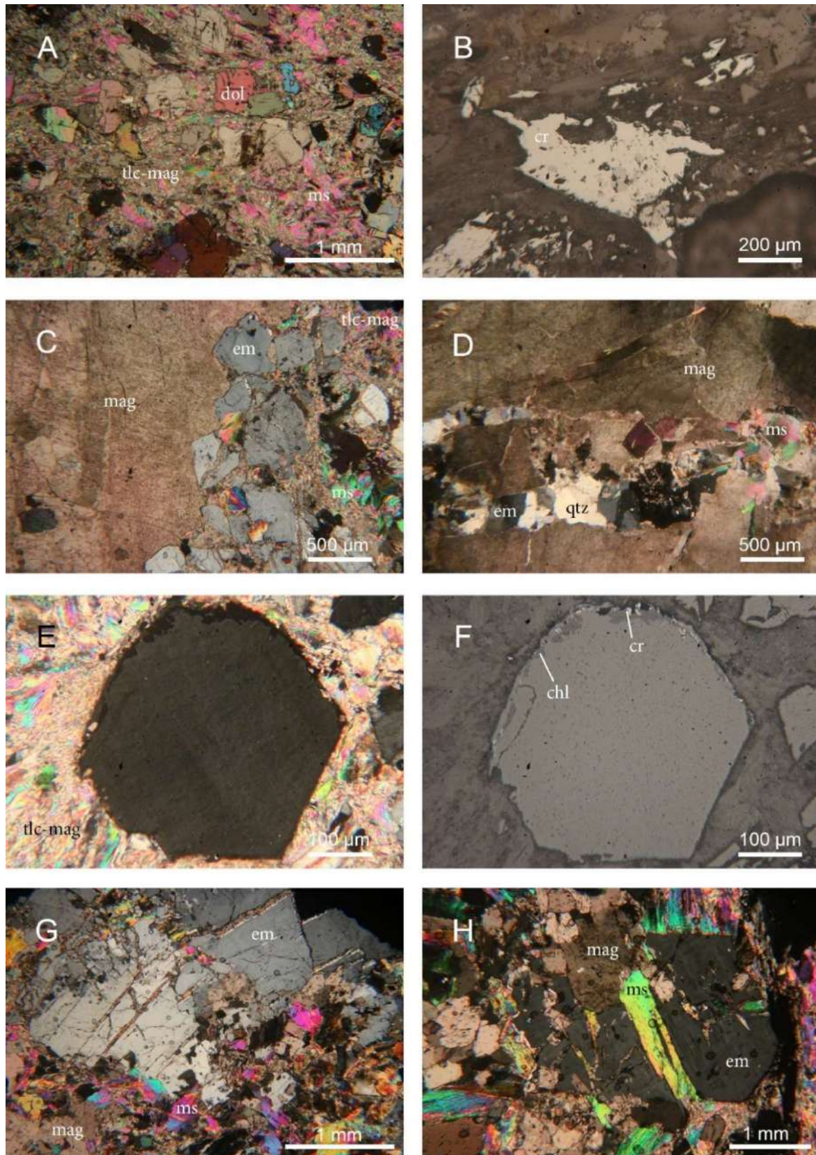
Figure 25: Thin sections. A An unmineralized section of host rock; microboudin or isolated dolomite grains occurring along schistosity planes in a fine interbedded magnesite-talc-muscovite matrix (LC-khalid-5, XPL). B A chromite grain inside the magnesite-talc matrix; note the salmon-grey opaque inclusion mineral, which could be pyrrhotite (LC-khalid-6, RL). C Emerald mineralization (dark gray first-order) found in a fine magnesite-talc-muscovite matrix, at the interface with large grained magnesite (LC-khalid-8, XPL). D Emerald-quartz-muscovite veinlet cross-cutting large-grained magnesite (LC-khalid-8, XPL). E Basal section of emerald in a fine magnesite-talc matrix. Some pinpoint mica inclusions in the emerald are visible
