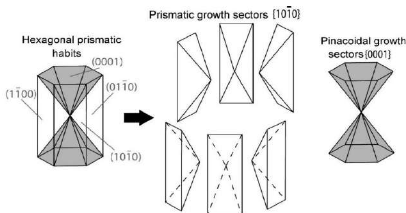
Figure 1: The common prismatic habit of beryl, with the 6 prismatic and 2 pinacoidal crystal faces and the different related growth sectors (Giuliani et al., 2019).
