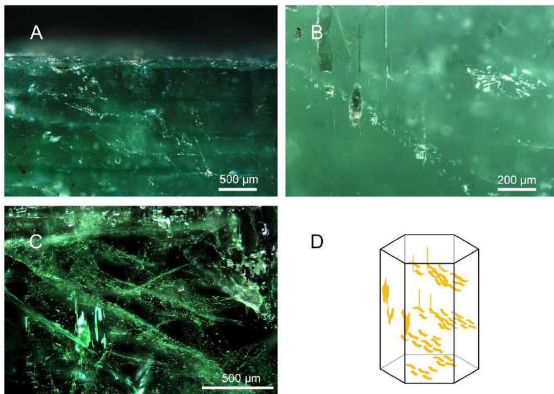
Figure 17: Primary, secondary and pseudosecondary fluid inclusions. A Pseudosecondary fluid inclusions arranged on parallel planes and secondary on the cleavage planes (FN12970, ethanol, darkfield). B Growth tubes, elongated chlorite sheets, «curved arrangement spreading on basal cleavage» (Gübelin and Koivula, 1997) of secondary fluids inclusions (right) (FN12974, ethanol, brightfield). C Jagged fluid plane (left), zigzag line (bottom left), secondary diagonal inclusions, smaller growth tubes, primary inclusions and a batch of small xenomorph transparent crystals (FN12969, ethanol, darkfield). D Sketch illustrating the inclusions sets found in Mingora emeralds.
