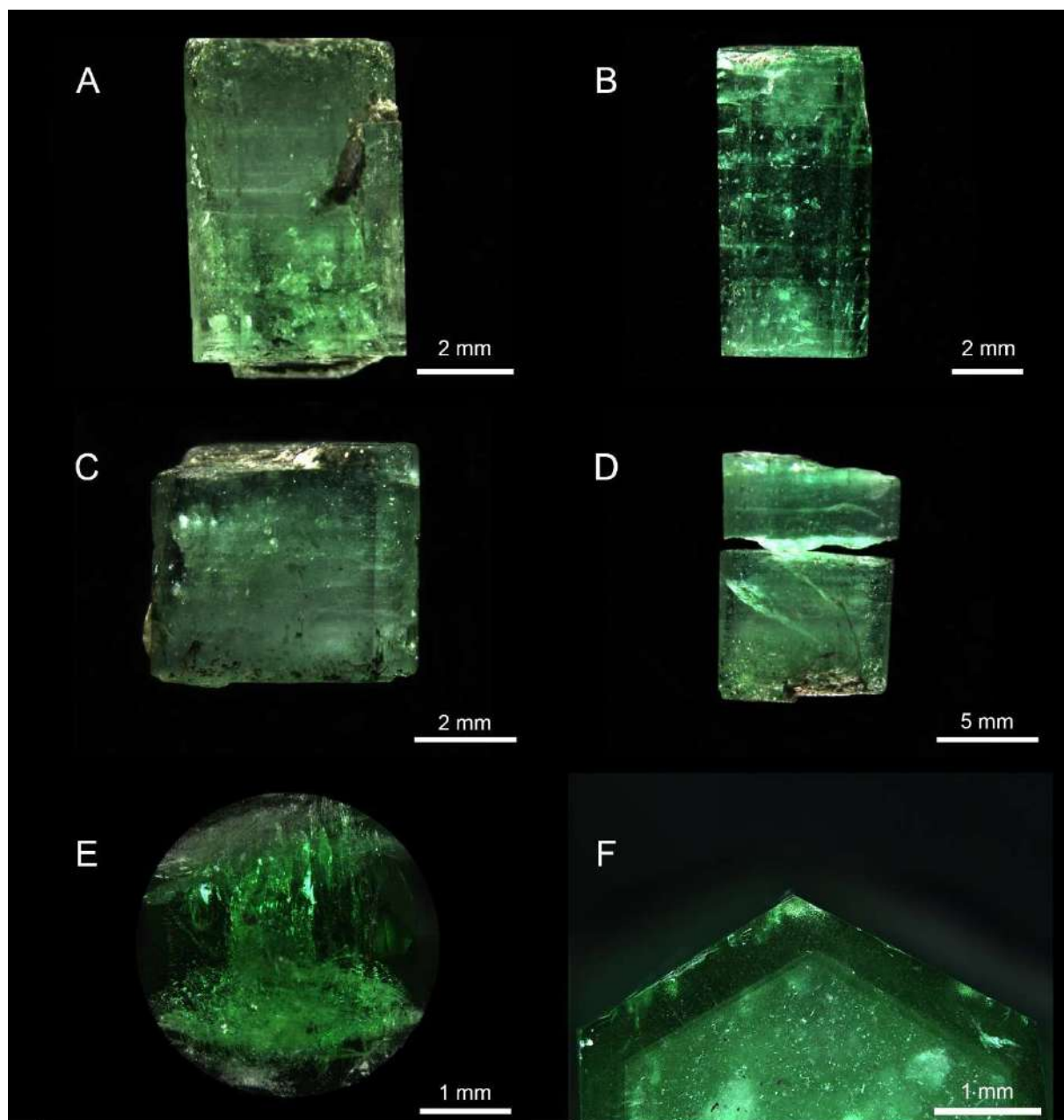
Figure 19: Zonation A Two growth sectors; a pinacoidal fuzzy growth sector with micas and fluid inclusions (top and core), and a more translucent hexagonal prismatic sector with qtz-dol (bottom), talc overplating (FN12969, ethanol, darkfield). B Two well-defined fuzzy pinacoidal growth sectors with micas (top and bottom) and a transparent hexagonal prismatic growth zone in the middle of the crystal (FN12491, ethanol, darkfield). C A more translucent and saturated sector overgrowing on the bottom fuzzy core (FN12974, ethanol, darkfield). D Sample with a fuzzy sector (bottom) and a fractured translucent top, broken at the limit during preparation (FN12970, ethanol, darkfield). E Small brilliant-cut emerald displaying an uneven color distribution (from culet, FN12984, ethanol, darkfield). F Sharp color and mineralogical distribution, 1C view (FN12491, ethanol, darkfield).
