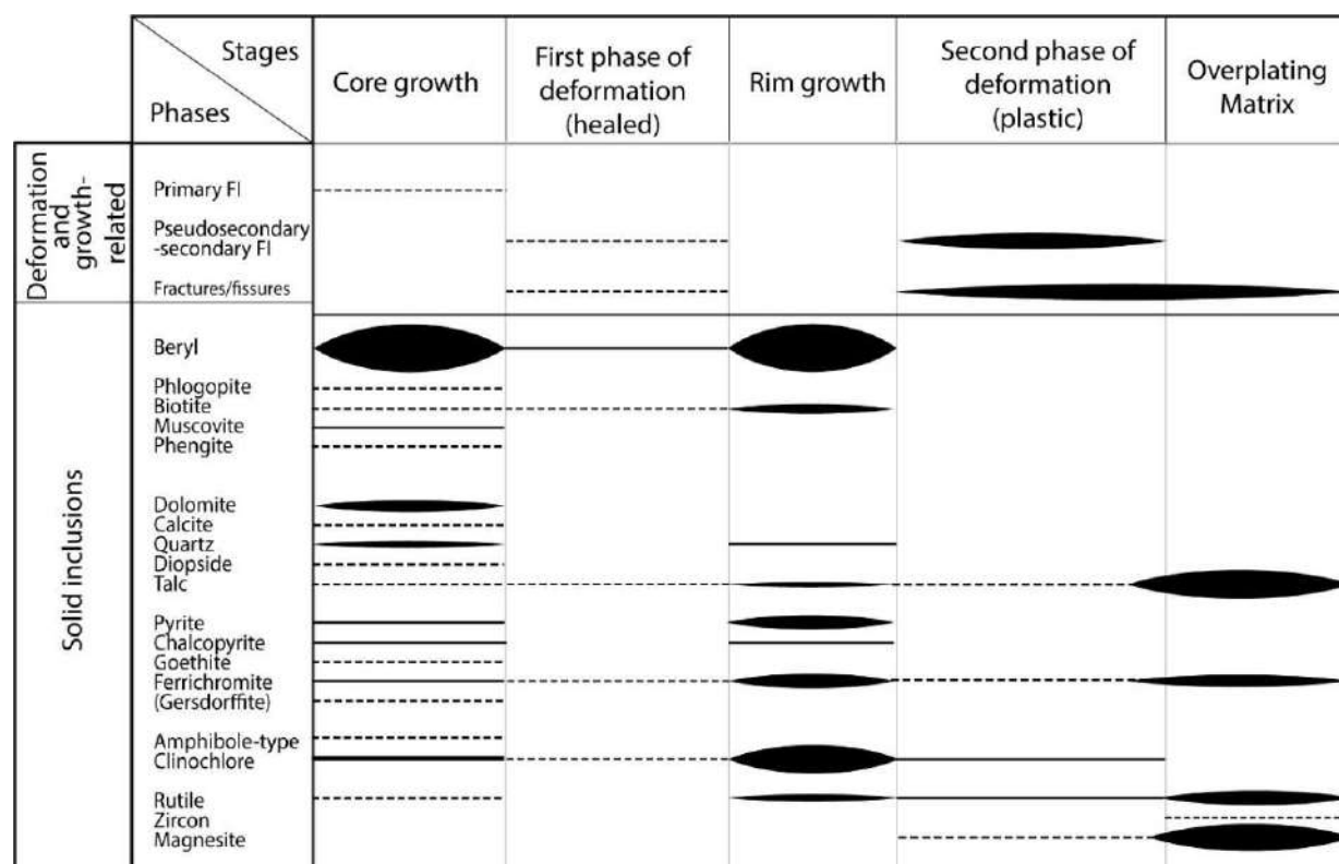
Figure 26: Paragenetic diagram. This diagram is the result of the merging of the paragenetic diagrams for each sample and is based on the distribution of the inclusions observed with the different methods.
