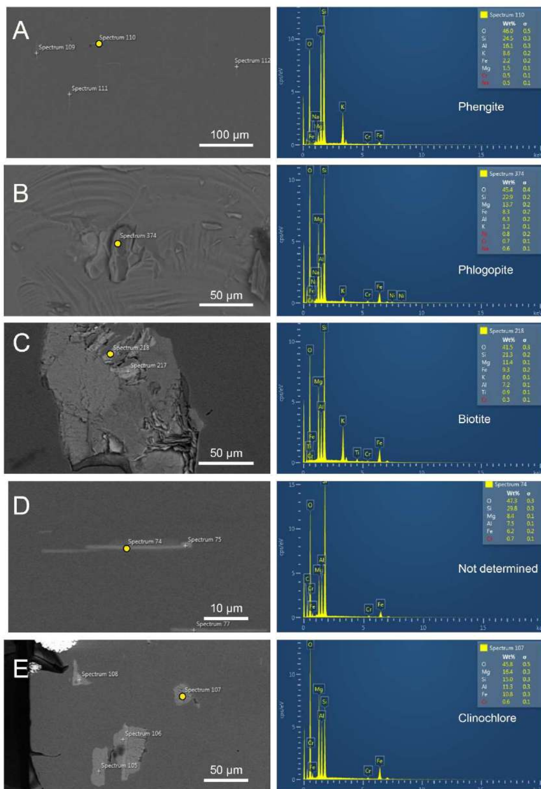
Figure 45: BSE pictures and compositions of inclusions in emerald samples. A Small perpendicular intersecting sheets of phengite (FN12974, BSE, polished). B Phlogopite occurring as thin stacked platelets (FN12970, BSE, crushed). C Soft biotite piles with titanium traces scratched away during polishing (FN12969, BSE, polished). D Undefined thin sheets of a mineral in composition between phyllosilicates and amphiboles (FN12974, BSE, polished). E Near the crystal face, (Cr-)clinocllore inclusions occurring with phlogopite (FN12974, BSE, polished).
