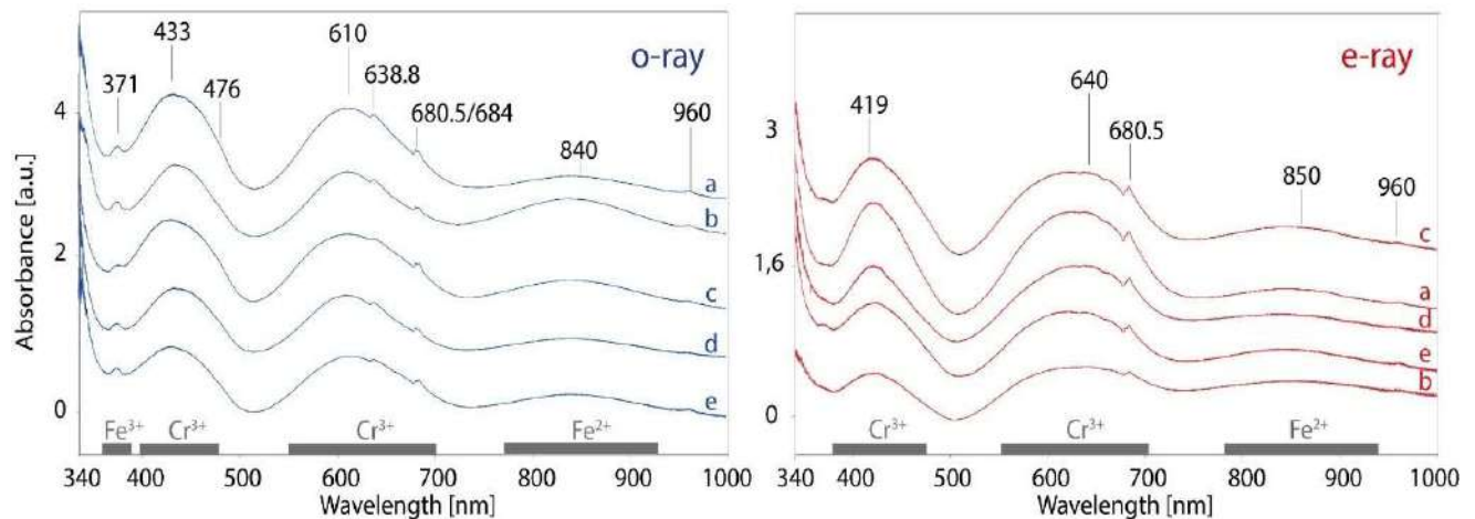
Figure 21: UV-Vis-NIR spectra of 5 samples, revealing the optical features of Mingora emeralds. The axes are set according to Smith (2009).
