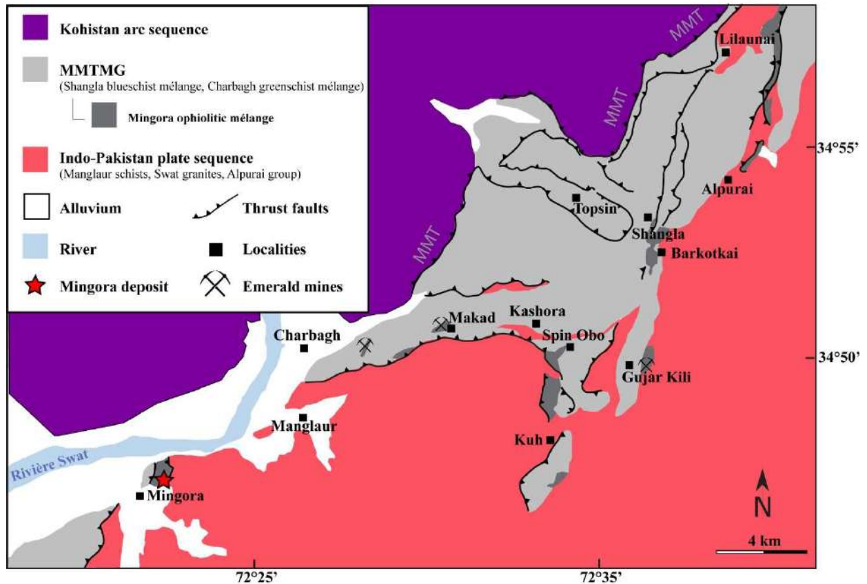
Figure 6: Tectonic map of the Mingora-Lilaunai area (after Arif and Moon, 2007, modified).
