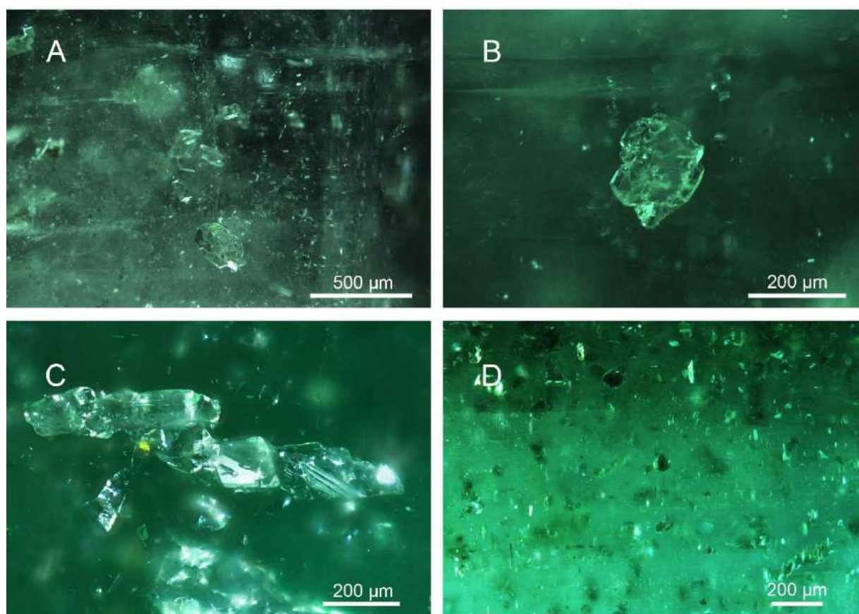
Figure 13: Solid inclusions (mica group and dolomite). A Group of «sharp dolomite crystallites» (Gübelin and Koivula, 1997) with few of them formed as perfect rhombohedral. They are occurring within a cloud of minute fluid inclusions and platy columnar micas (FN12491, ethanol, darkfield). B Potential dolomite twinning (FN12491, ethanol, darkfield). C Cluster of sharp dolomite rhombohedra (FN12973, ethanol, darkfield). D Darker cloud of platy columnar phlogopite (FN12970, ethanol, brightfield).
