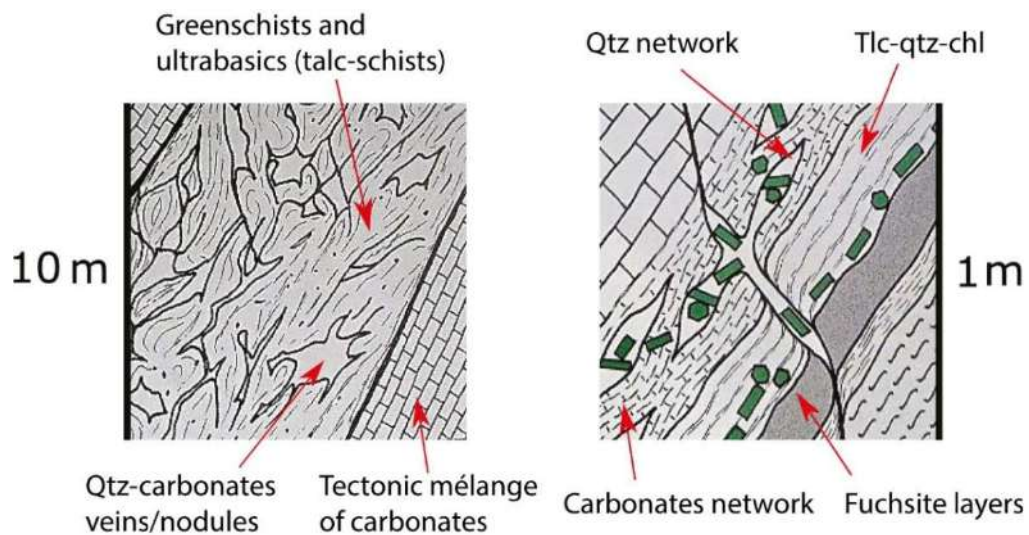
Figure 7: Model of "Schists without pegmatites: Emerald in carbonate-talc-schists and quartz lenses" for Swat, Pakistan (Schwarz, 2002, modified). Overview (left) and details (right).
