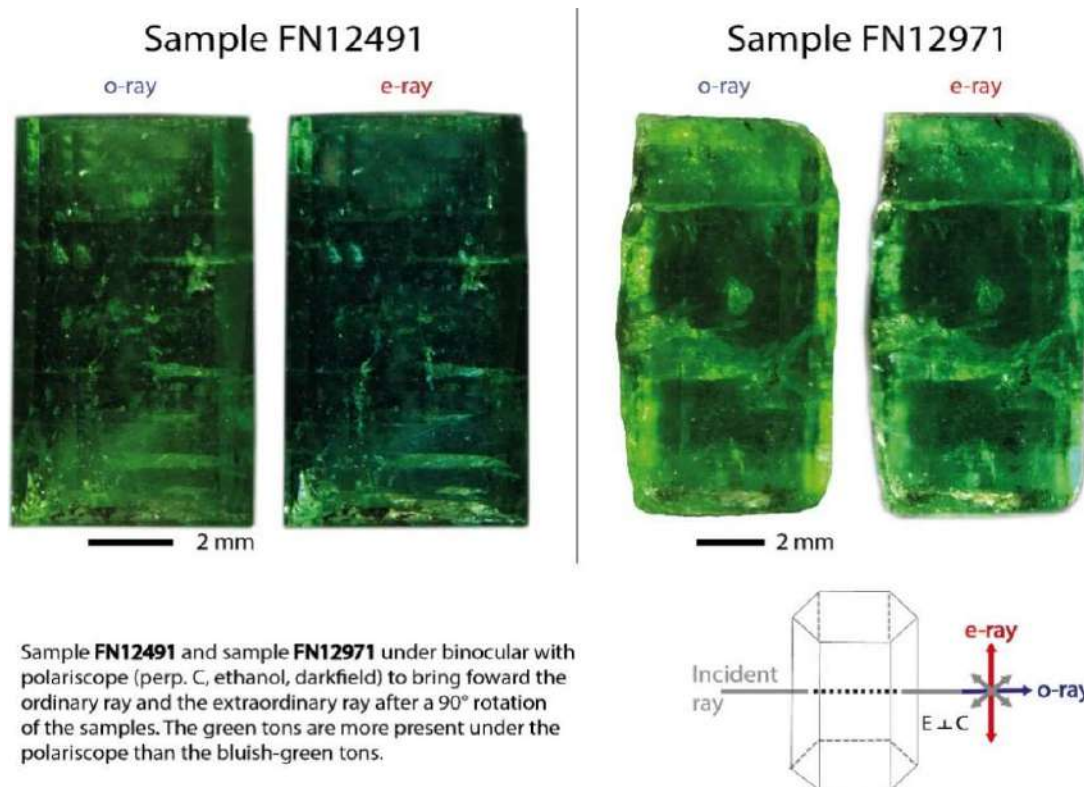
Figure 11: Pleochroism of the emerald samples
