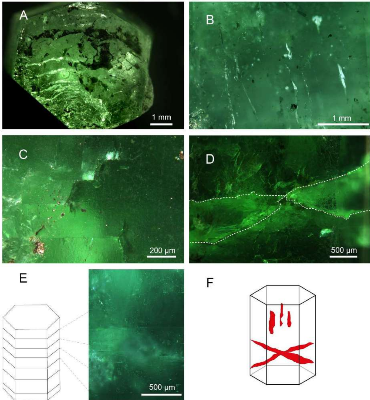
Figure 18: Fractures. A Basal concentric fractures with no related solid inclusions inside (FN12974, ethanol, darkfield). B Wavy fractures parallel to the C-axis with no related solid inclusions inside (FN12974, ethanol, darkfield). C Diagonal fractures shifted by the cleavage plane and its «flat parallel fissures» (Kazmi and Snee, 1990) (FN12975, ethanol, darkfield). D Set of conjugated shear fractures crossing the prismatic faces (FN12971, ethanol, darkfield). E Cleavage planes, not discernible in every samples (FN12941, ethanol, darkfield). F Sketch illustrating the fractures found in the Mingora emeralds.
