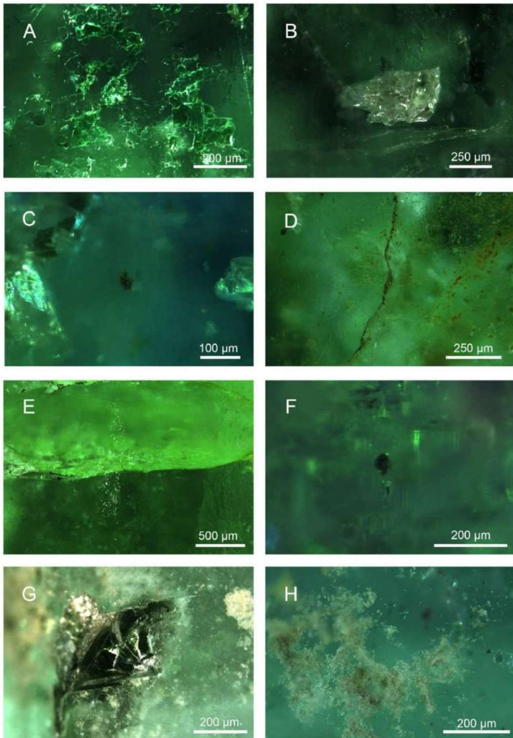
Figure 28: A Rounded or geometrical chlorite sheets (FN12969-7, ethanol, darkfield). B An anhedral dolomite crystal (FN12969-8, ethanol, darkfield). C Granular brown aggregates (FN12969-9, ethanol, darkfield). D A undulating surface-reaching late fracture, parallel to C-axis (FN12969-11, ethanol, darkfield). E A late fracture cross-cutting a primary fluid inclusions plane (FN12971-3, ethanol, darkfield). F Small unidentified platy dark mineral surrounded by blocky fluid inclusions (FN12972-3, ethanol, darkfield). G Overplating chlorite (FN12973-2, air, brightfield). H Beige mossy rutile aggregate (FN12973-4, ethanol, brightfield).
