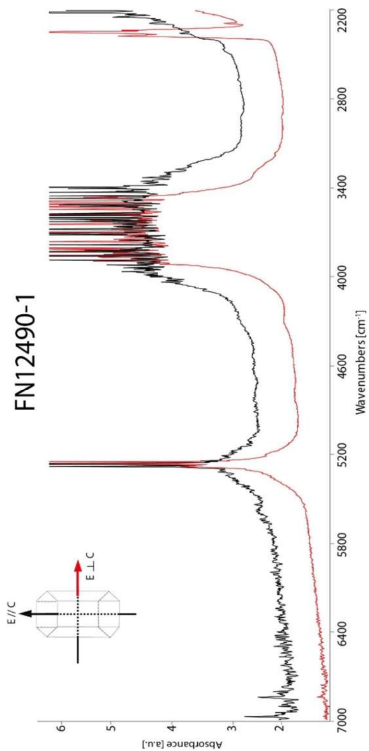
Figure 37: Absorbance IR spectrum for FN12490-1 sample.
