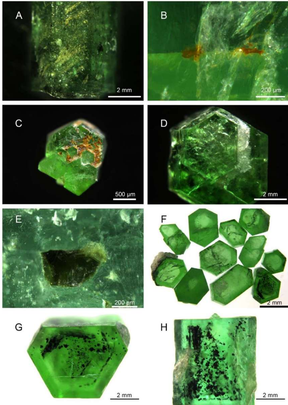
Figure 20: Introduction timing. A Yellow rutile aggregates on a prismatic face spreading as diagonal trails, following the same angle as some of the fluid inclusions (FN12969, ethanol, darkfield). B Orange rutile aggregates formed at the interface of a cleavage plane (FN12972, ethanol, darkfield). C Pinacoidal faces of an emerald cluster, sprinkled with orange rutile aggregates and talc-magnesite (FN13156, ethanol, darkfield). D Microcrystalline magnesite on the pinacoidal face (FN12978, ethanol, darkfield). E Outcropping of dark green platy chlorite on an unpolished prismatic face (FN12977, ethanol, darkfield). F Smaller crystals displaying lighter colors in the core than on the rims. Note the residual talc-magnesite host rock left on some crystals (FN13155, ethanol, brightfield). G-H (pinacoid face-prismatic face) A piece of the previous lot illustrating the color disparities and chromite flakes in specific zones (FN13155, ethanol, brightfield).
