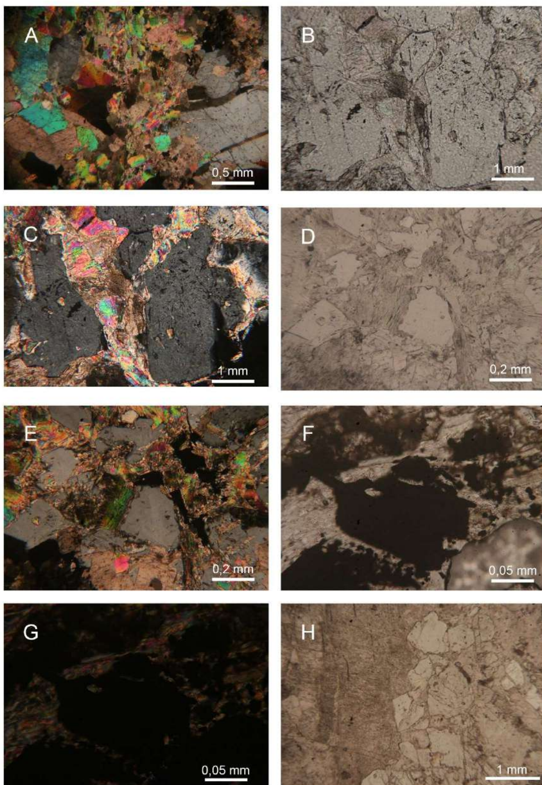
Figure 40: A General view (LC-khalid-6, XPL). B Diverse emerald crystals with inclusions in tlc-mag matrix (LC-khalid-6, PPL). C Same emerald crystals with some visible micas inclusions (LC-khalid-6, XPL). D (Micaceous)-tlc matrix enclosing emerald crystals (LC-khalid-6, PPL). E Same view in crossed polar (LC-khalid-6, XPL). F A chromite grain disseminated in the magnesite-talc (LC-khalid-6, PPL). G Same grain (LC-khalid-6, XPL). H The emerald mineralization in a fine magnesite-talc-muscovite matrix, at the interface with the large grained magnesite (LC-khalid-8, PPL).
