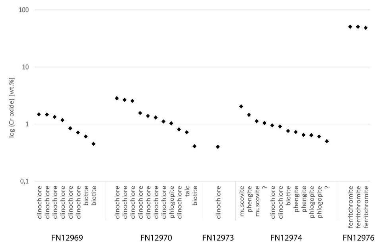
Figure 49: log Cr-oxide concentration in Cr-bearing inclusions, analyzed by EDX-SEM
