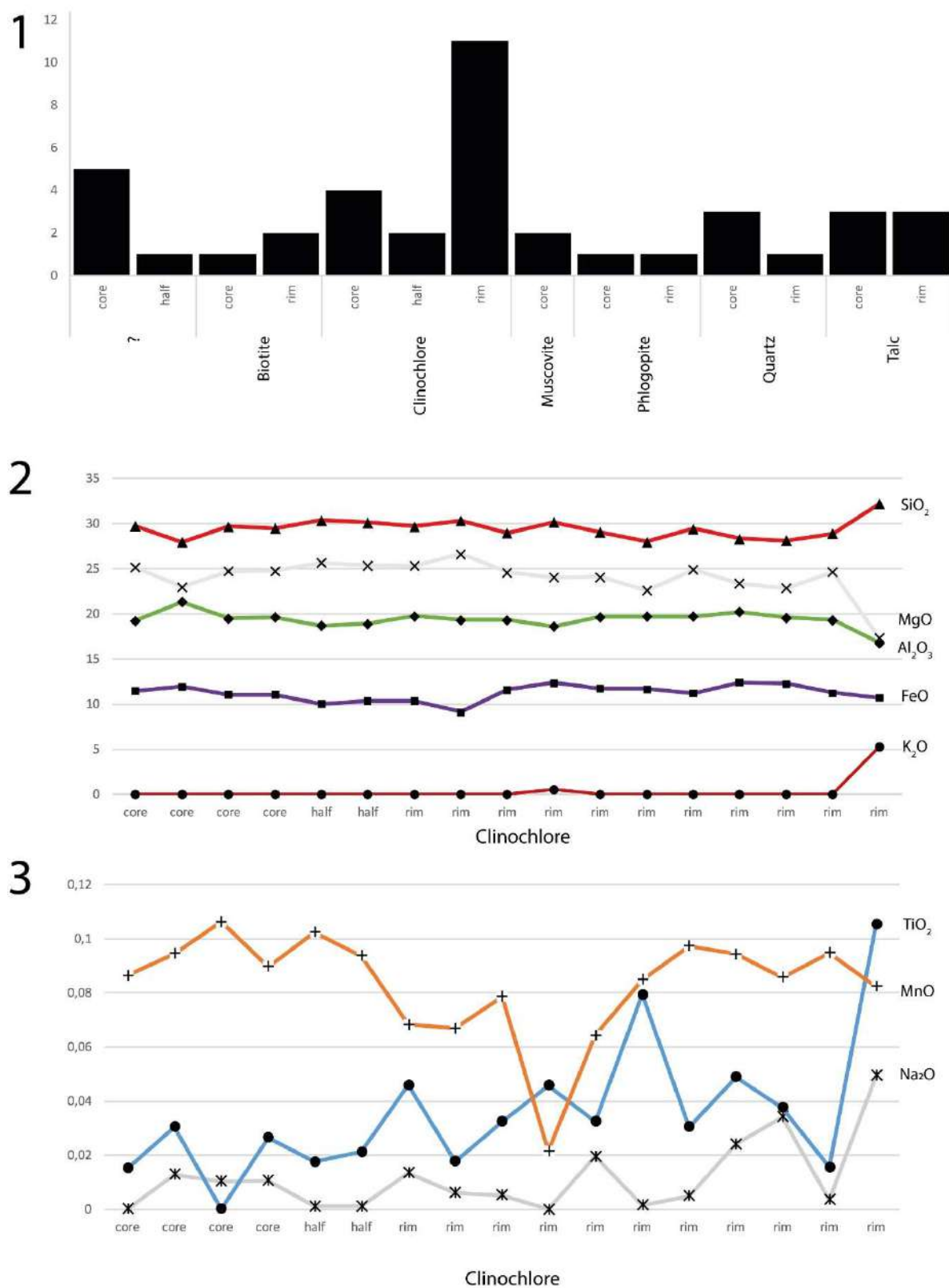
Figure 51: 1) Core, half-way, rim sectors and the relative distribution of the inclusions analyzed by microprobe. 2) Major elements concentrations in the samples analyzed by microprobe, organized by sector. 3) Minor (and trace) elements in concentrations in the samples analyzed by microprobe, organized by sector.
