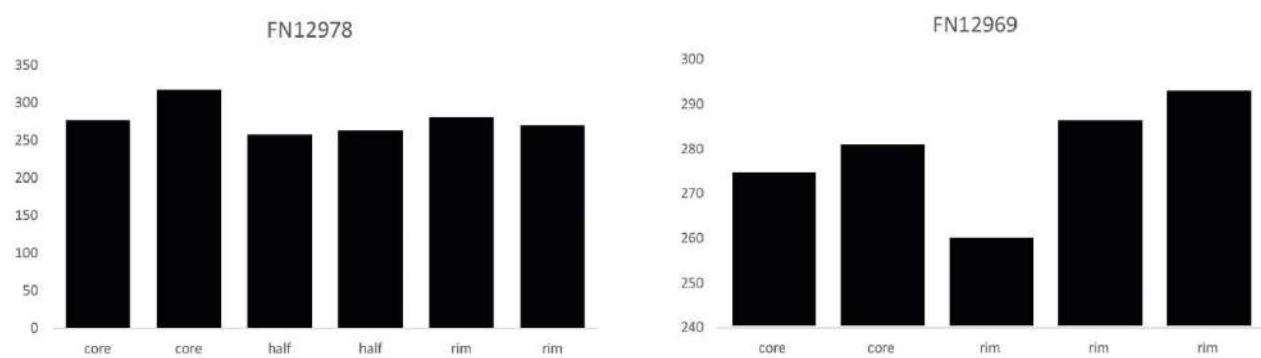
Figure 50: Chlorite temperatures (Cathelineau, 1988). The distribution between the core and the rim are homogenous and do not show a temperature gradient
