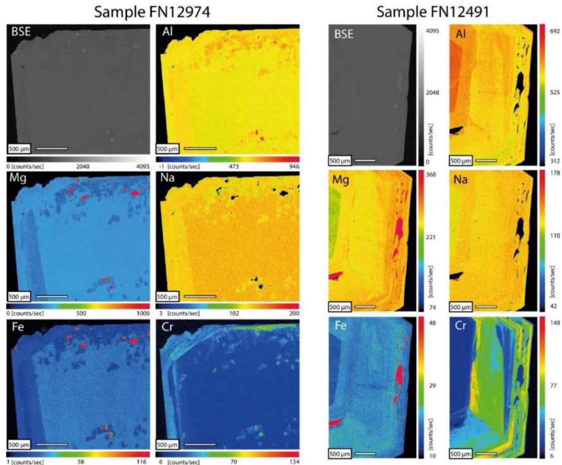
Figure 24: Microprobe chemical maps of FN12974 and FN12491 samples
