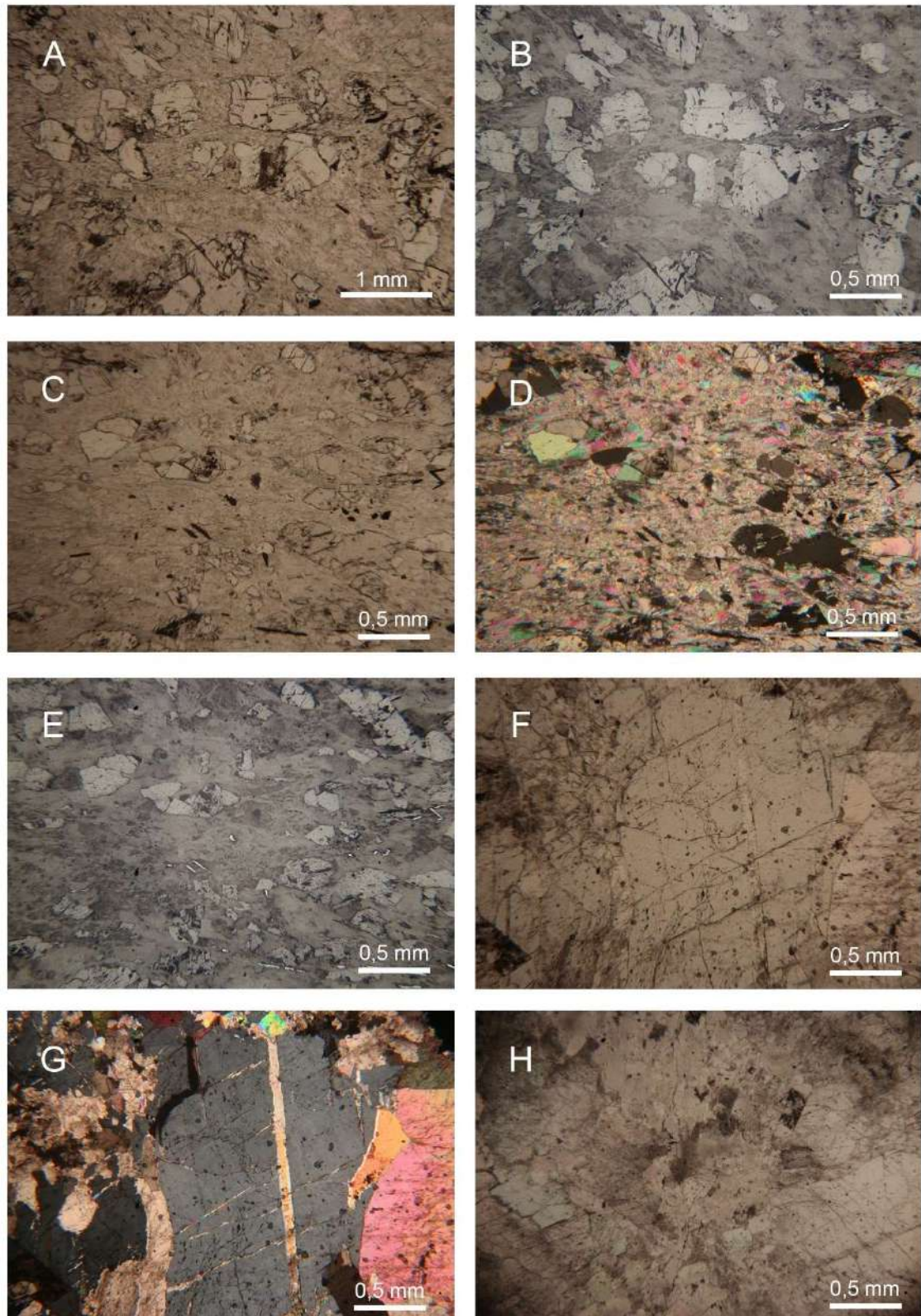
Figure 39: A Unmineralized section of host rock; microboudin or isolated dolomite grains occur along schistosity planes in a fine interbedded magnesite-talc-muscovite matrix (LC-khalid-5, PPL). B Same section in reflected light (LC-khalid-5, RL). C Another view of the unmineralized section of host rock (LC-khalid-5, PPL). D Same view (LC-khalid-5, XPL). E Same view, note some elongated light-grey grains of chromites (following foliation S-planes?) (LC-khalid-5, RL). F A fractured emerald crystal (LC-khalid-6, PPL). G A fractured emerald crystal with intrusive magnesite along cleavage planes and fractures (LC-khalid-6, XPL). H General view (LC-khalid-6, PPL).
