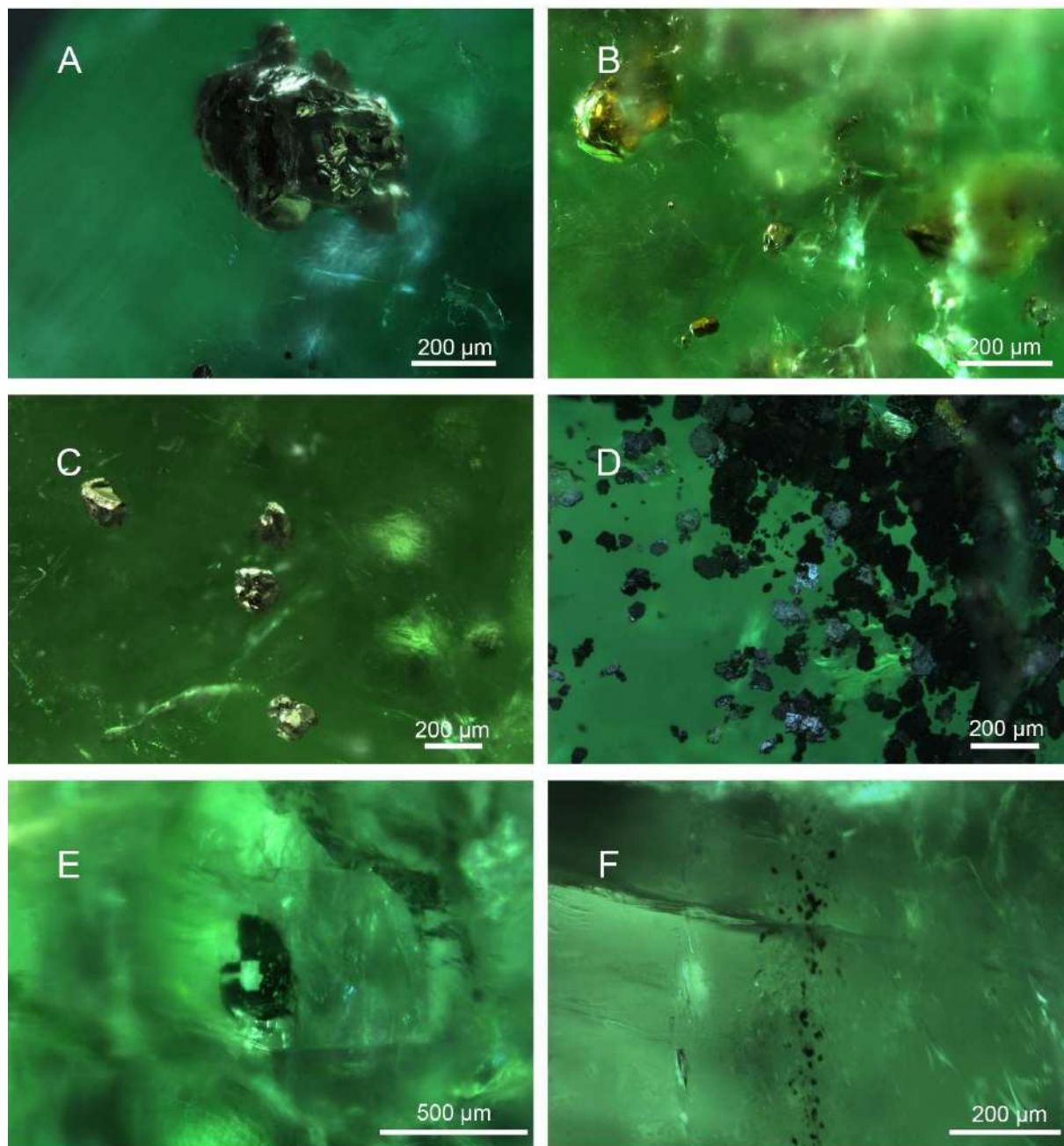
Figure 15: Solid inclusions (oxides and sulfurs). A Rounded polyhedral pyrite grain (FN12975, ethanol, darkfield). B Cluster of sulfurs, composed of pyrite and chalcopyrite, based on the reflectance and the color (FN12975, ethanol, darkfield). C Cluster of pyrite grains, with some having a modified dodecahedron shape (FN12975, ethanol, darkfield). D Batch of «sharp chromite» flakes (Gübelin and Koivula, 2008; Kazmi and Snee, 1990) (FN12976, ethanol, darkfield). E Rare small thin perforated circle. Kazmi and Snee (1990) or Gübelin and Koivula (2008) described similar forms as either pyrrhotite or Cr-film (FN12978, ethanol, darkfield). F Patches of unidentified opaque minerals, gersdorffite lookalike, as described in Kazmi and Snee (1990) (FN12984, ethanol, darkfield).
