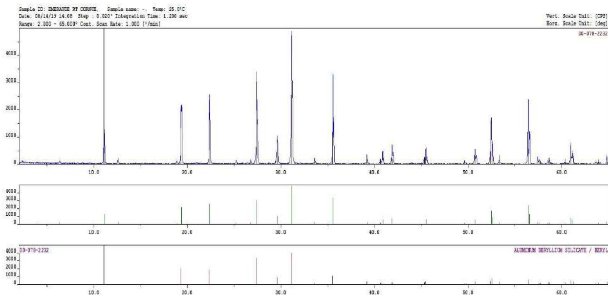
Figure 42: ED-XRD pattern on FN12970 fine-crushed powder. Note the major diffraction peaks of emerald and only few smaller peaks indicate the presence of chlorite group minerals.
